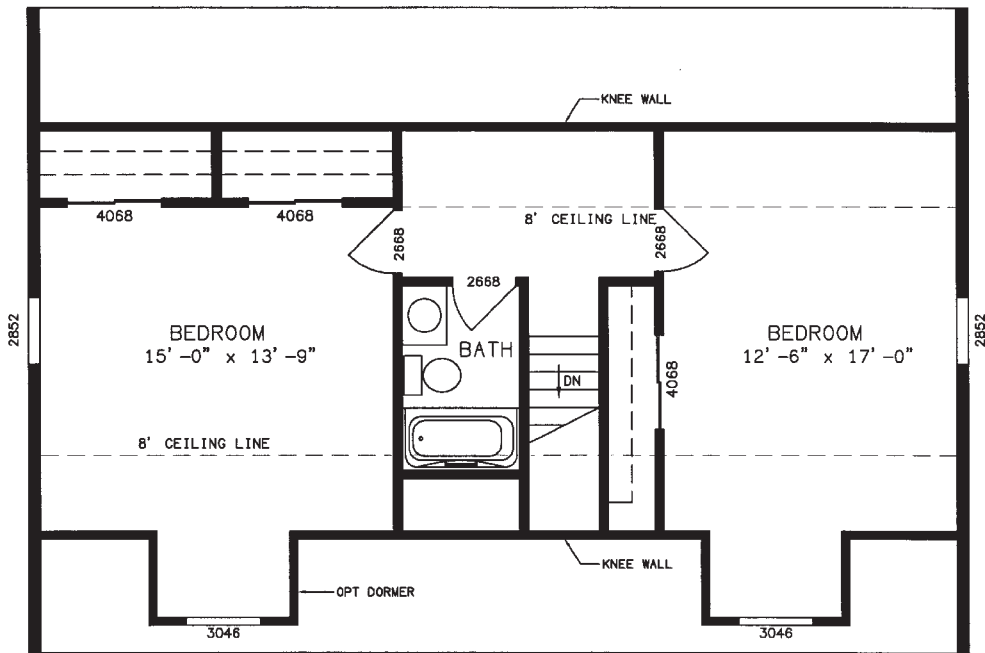
PLAN NO. VC3871 PROPOSED SECOND FLOOR (BY OTHERS) 17'0" X 40'0"
