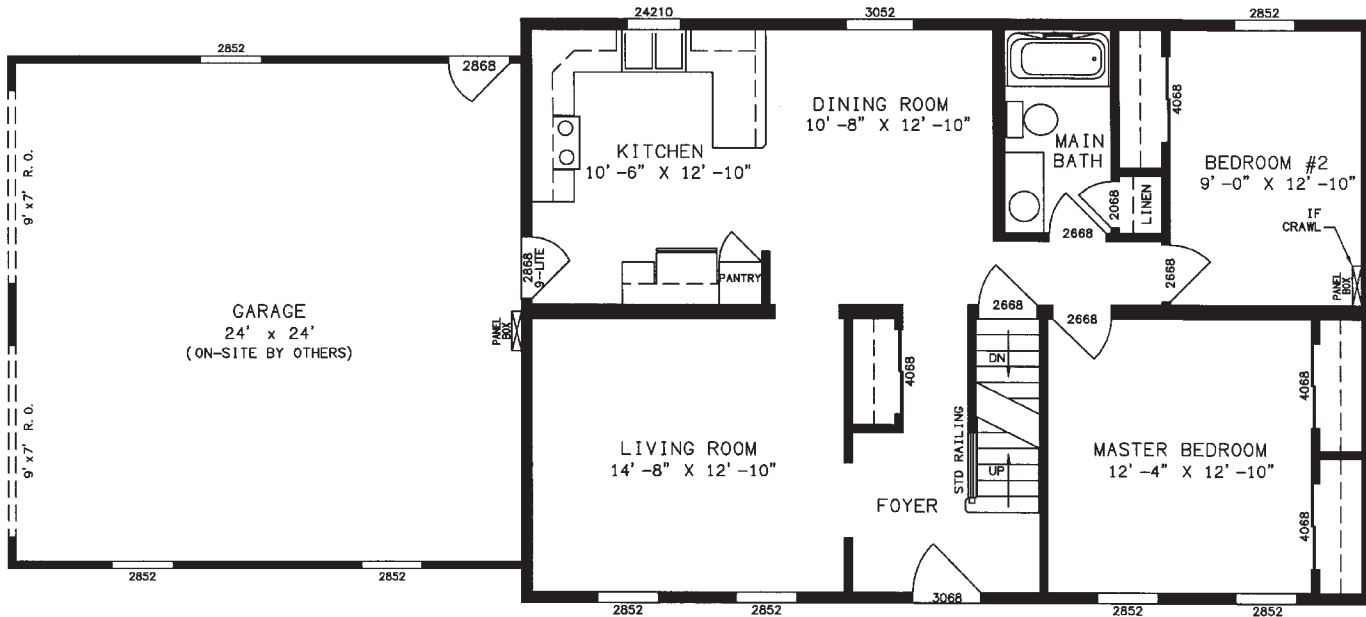
PLAN NO. VC3871 27'4" X 40'0" 1093 sq. ft.
