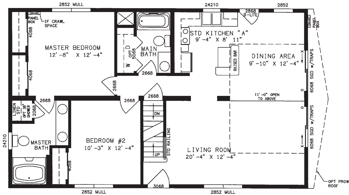
PLAN NO. VC3521 26'4" X 44'0" 1159 sq. ft.
