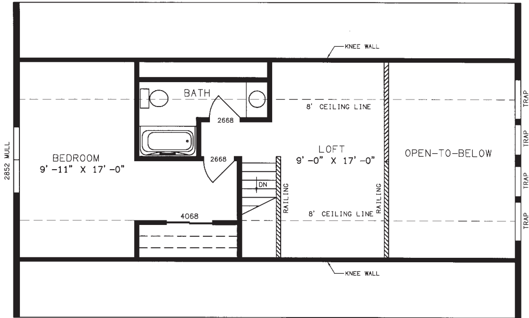
PLAN NO. VC3521 PROPOSED SECOND FLOOR (BY OTHERS) 17'0" X 44'0"
