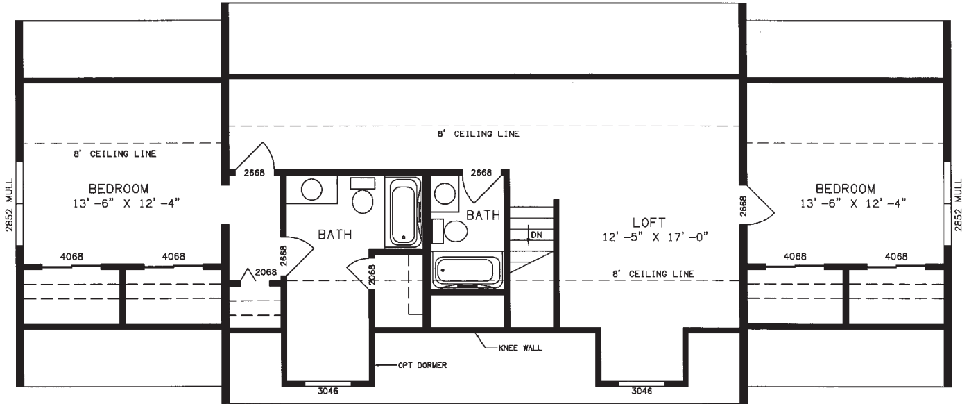
PLAN NO. VC3870 PROPOSED SECOND FLOOR (BY OTHERS) 17'0"/11'5" X 64'0"
