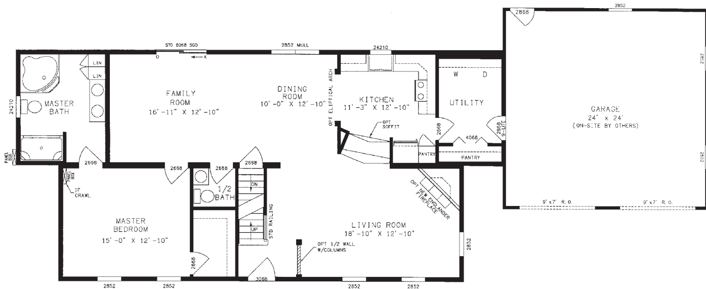
PLAN NO. VC3902 FIRST FLOOR 27'4" X 48'58" 1448 sq. ft.
