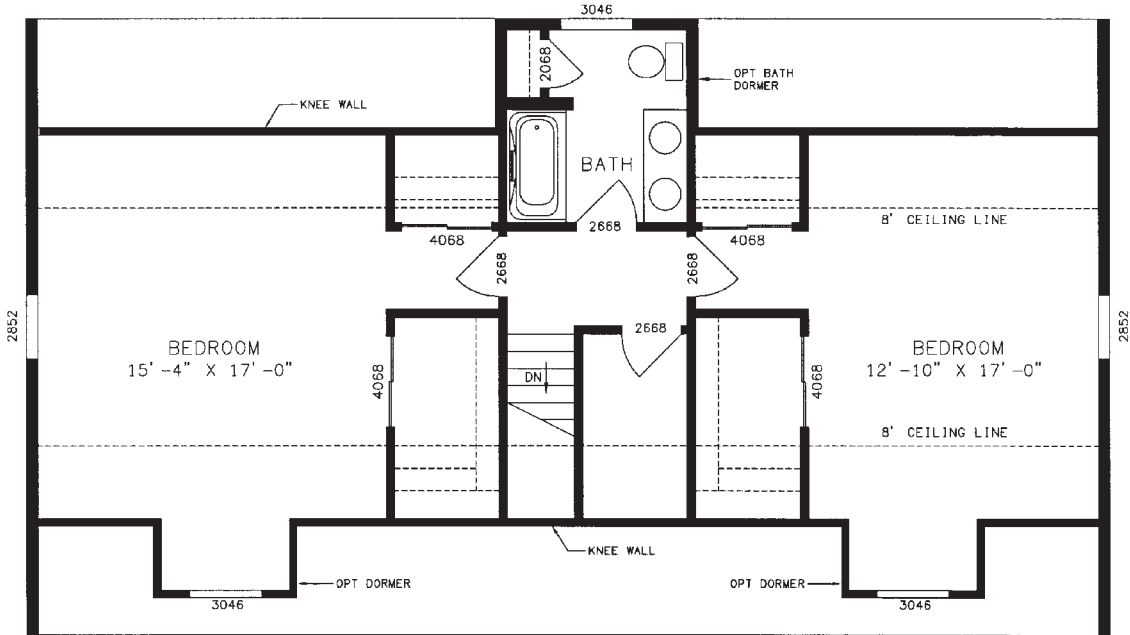
PLAN NO. VC3902 PROPOSED SECOND FLOOR (BY OTHERS) 17'0" X 48'0"
