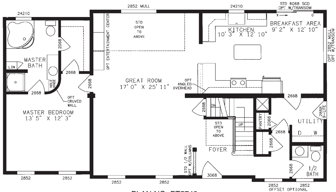
PLAN NO. PT5748 FIRST FLOOR 27'4"/25' X 52'0" 2426 sq. ft.
