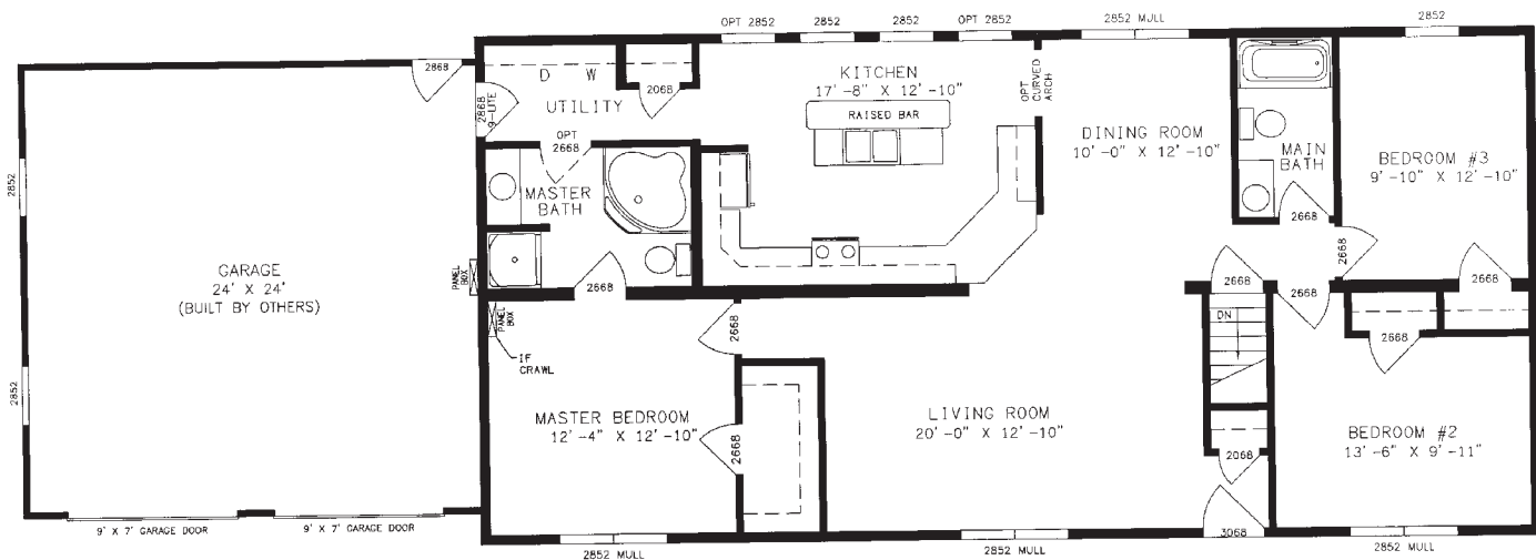
PLAN NO. MR2745 27'4" X 56'0" 1530 sq. ft.
