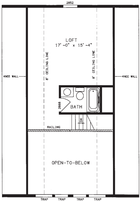
PLAN NO. VC3869 PROPOSED SECOND FLOOR (BY OTHERS) 17'0" X 38'0"
