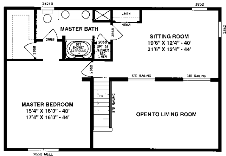
ASPEN II PLAN NO. PT5024 SECOND FLOOR 26'4" X 40'0"
