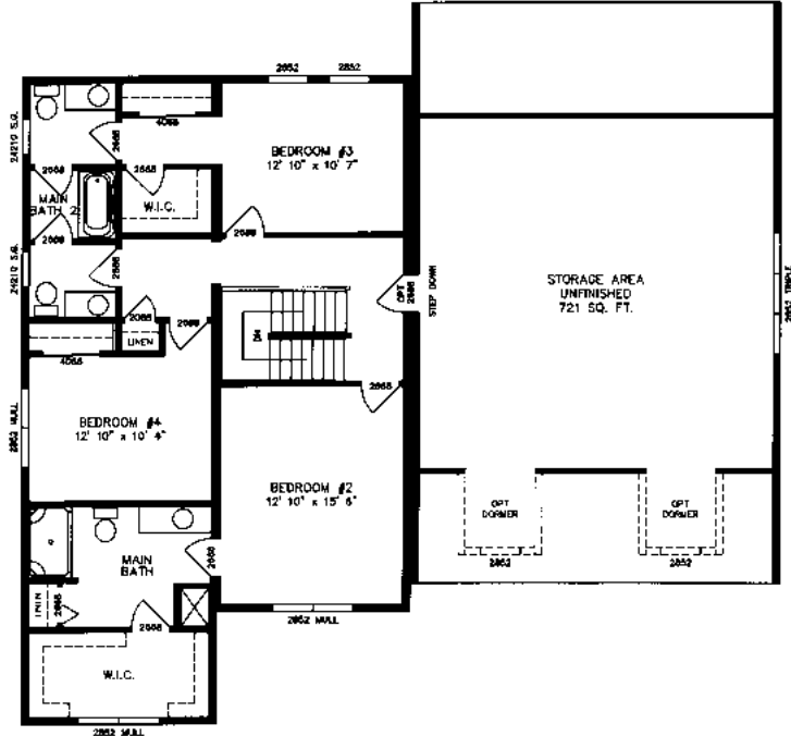
HAMPTON PLAN NO. LT0109 SECOND FLOOR 27'4" X 46'/38'0"
