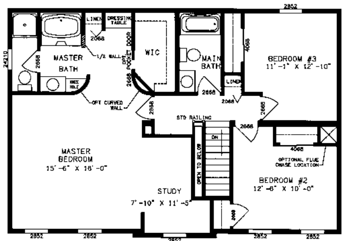
LEXINGTON PLAN NO. PT5729 SECOND FLOOR 27'4" X 40'0"/46'0"
