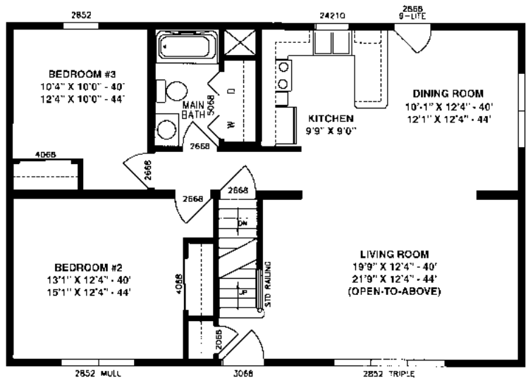
ASPEN I PLAN NO. PT5010 FIRST FLOOR 26'4" X 40'0" 2106 SQ. FT.
