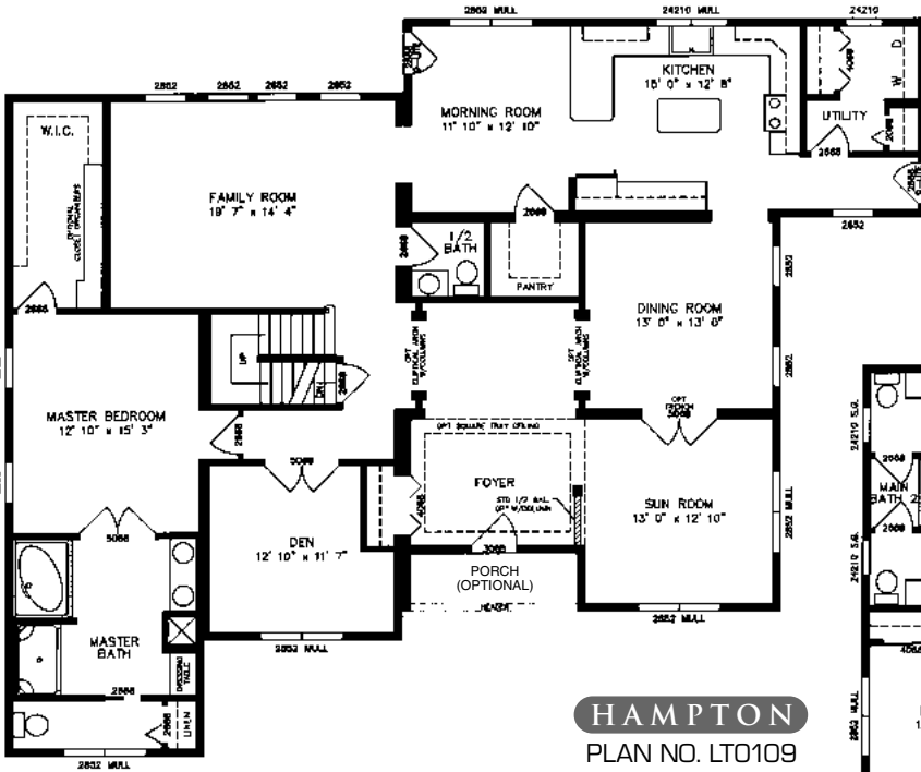
HAMPTON PLAN NO. LT0109 FIRST FLOOR 27'4" X 46'/38'0" 41'0" X 26'/36'0" 3457 SQ. FT.
