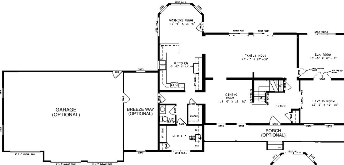
HARRISON PLAN NO. PT5705 FIRST FLOOR 27'4" X 55'9" 3502 SQ. FT.
