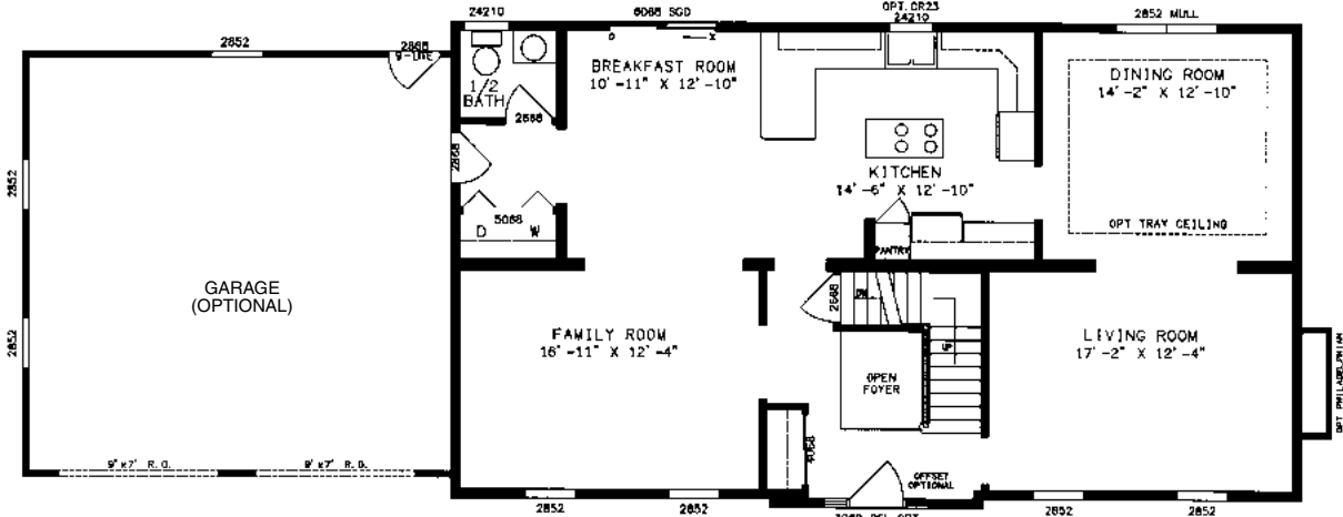
AMHERST PLAN NO. PT5736 FIRST FLOOR 27'4" X 48'0" 2576 SQ. FT.
