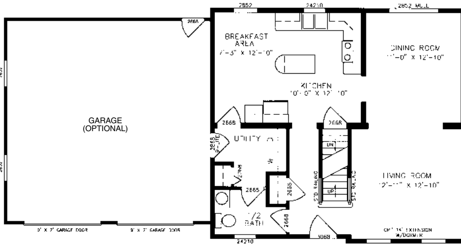
KEYSTONE PLAN NO. PT5701 FIRST FLOOR 27'4" X 30'0" 1640 SQ. FT.
