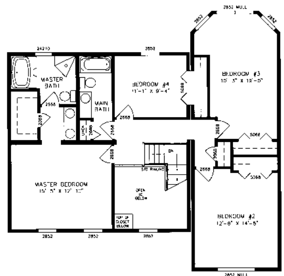
SALEM PLAN NO. PT5722 SECOND FLOOR 27'4" / 39'7" X 41'10"
