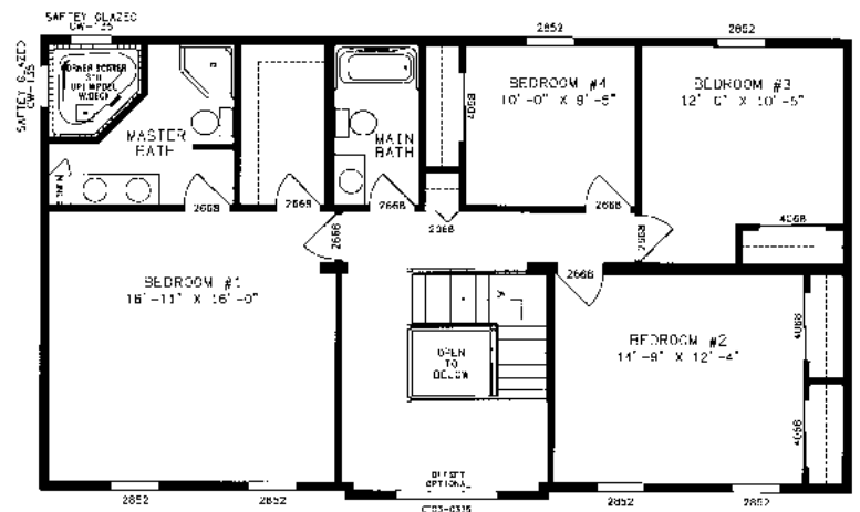
AMHERST PLAN NO. PT5736 SECOND FLOOR 27'4" X 48'0"
