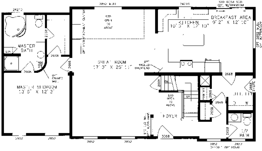
CHATHAM PLAN NO. PT5748 FIRST FLOOR 27'4"/25' X 52'0" 2426 SQ. FT.
