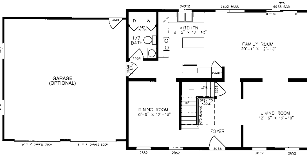
WESTON PLAN NO. PT5716 FIRST FLOOR 27'4" X 36'0" 1966 SQ. FT.
