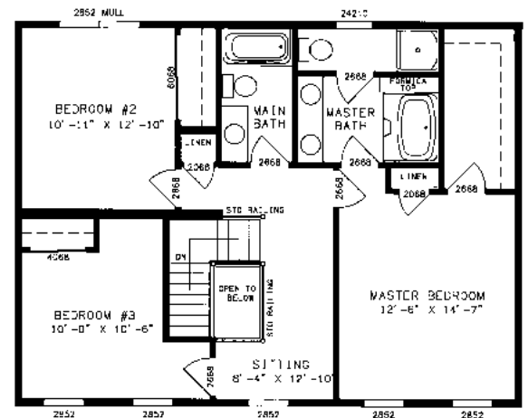
WESTON PLAN NO. PT5716 SECOND FLOOR 27'4" X 36'0"
