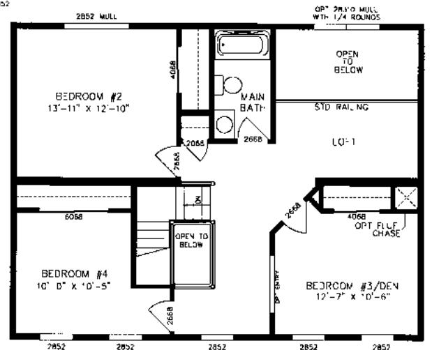
MONROE PLAN NO. PT5711 SECOND FLOOR 27'4" X 36'0"
