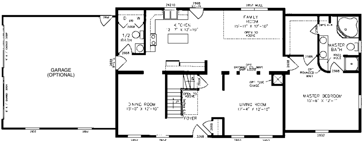
MONROE PLAN NO. PT5711 FIRST FLOOR 27'4" X 36'0" 25'0" X 16'0" 2366 SQ. FT.
