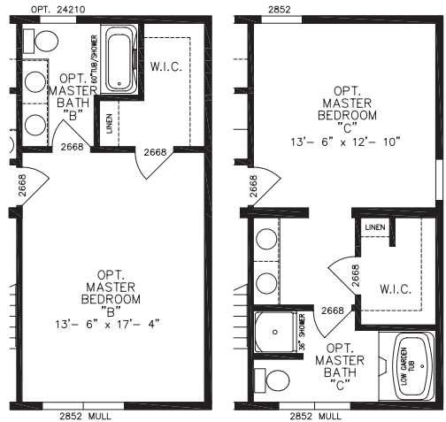
CHAMPLAIN PLAN NO. CS4035 27'4" X 38'0" 1041 SQ. FT.
