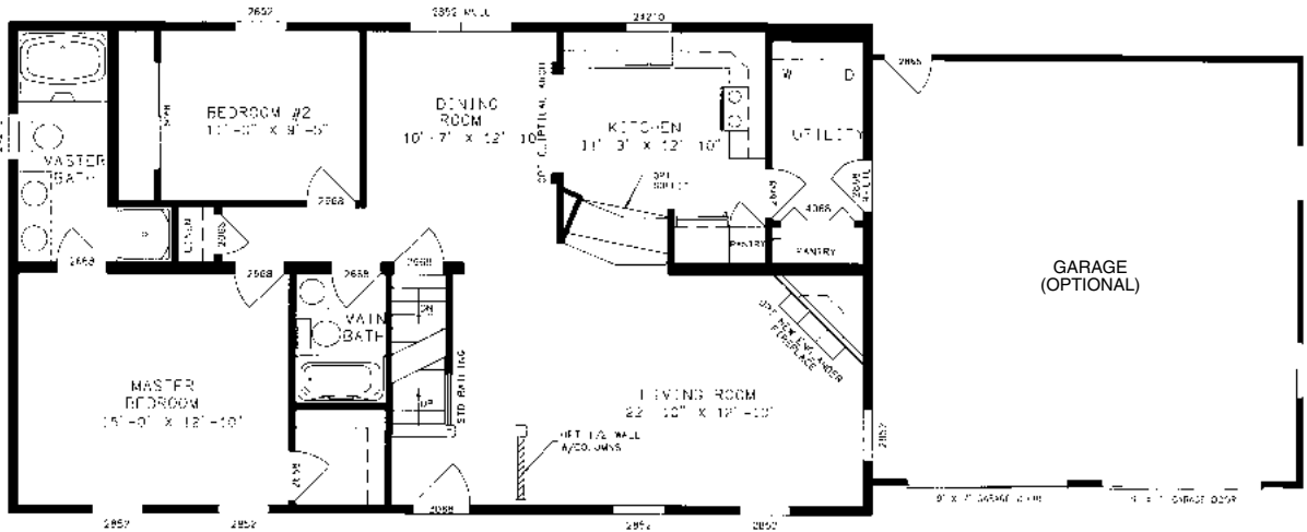
WARWICK PLAN NO. VC3867 27'4" X 48'0" 1312 SQ. FT.
