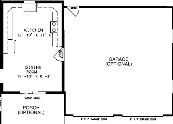
BRANDYWINE PLAN NO. VC3869 27'4" X 38'0" 13'8" X 27'4" 1411 SQ. FT.
