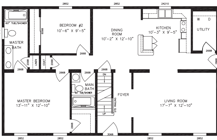
BELLAIRE PLAN NO. CS4036 27'4" X 46'0" 1257 SQ. FT.
