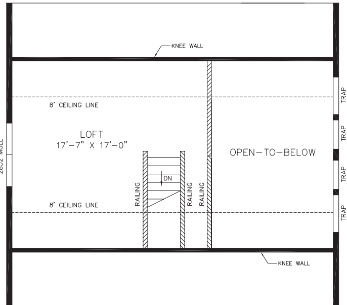
VALE PLAN NO. CS4030 FINISHED UPSTAIRS (OPTIONAL) 17'0" X 30'0"
