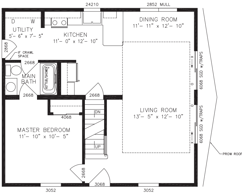
VALE PLAN NO. CS4030 27'4" X 30'0" 820 SQ. FT.
