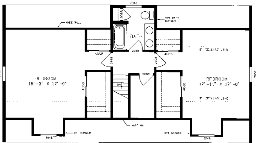
WESTMINSTER PLAN NO. VC3528 FINISHED UPSTAIRS (OPTIONAL) 17'0" X 48'0"
