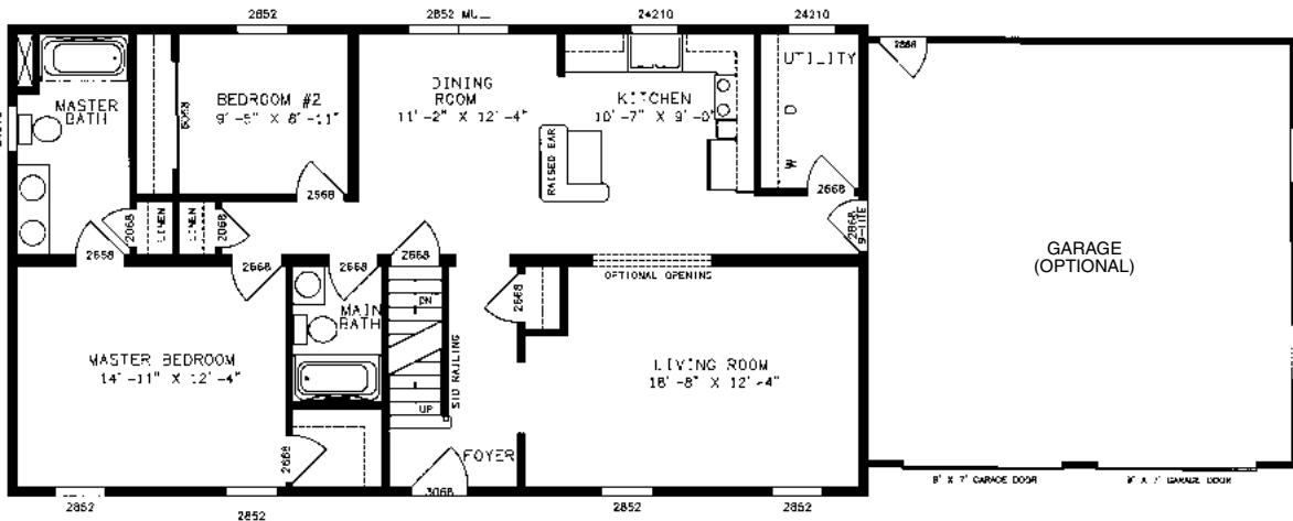
WESTMINSTER PLAN NO. VC3528 26'4" X 48'0" 1264 SQ. FT.
