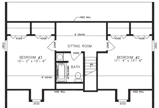
CHAMPLAIN PLAN NO. CS4035 FINISHED UPSTAIRS (OPTIONAL) 17'0" X 38'0"
