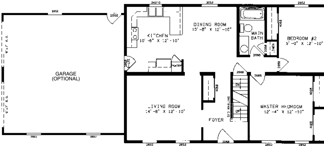
RALEIGH PLAN NO. VC3871 27'4" X 40'0" 1093 SQ. FT.
