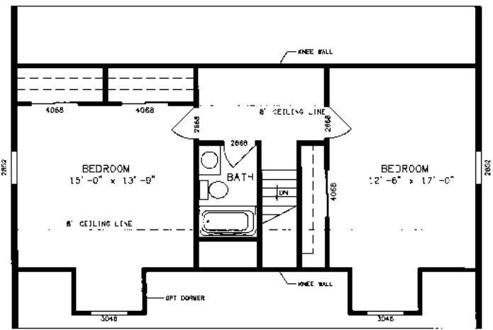
RALEIGH PLAN NO. VC3871 FINISHED UPSTAIRS (OPTIONAL) 17'0" X 40'0"
